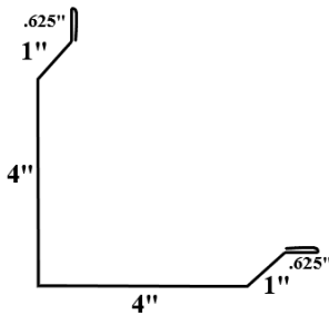
Horiz. Corner Post - Inside
