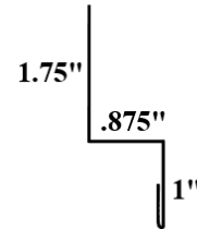
Eave Trim
