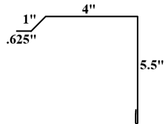
Inside Corner
