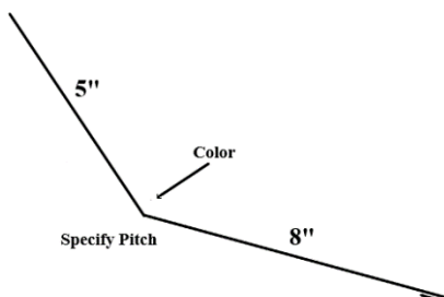
Pitch Change - Inside
