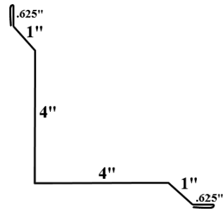
Horiz. Corner Post - Outside
