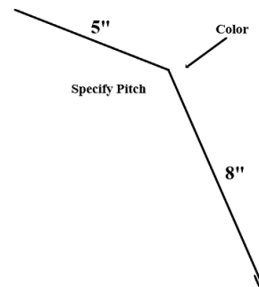
Pitch Change - Outside
