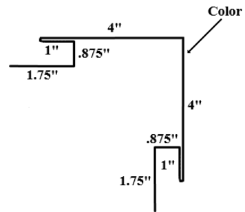
Horiz. Corner Post - Outside
