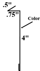
Snow Break
