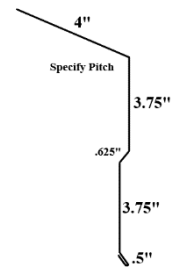
C-Flashing
