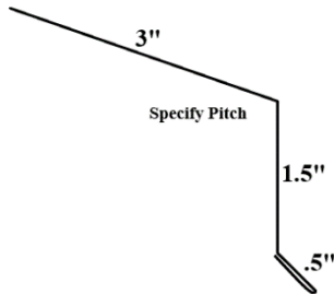
Z-Flashing
