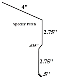
Eave
