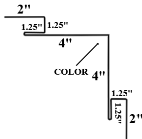
Horiz. Corner Post - Inside
