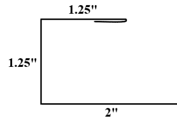
C-Flashing
