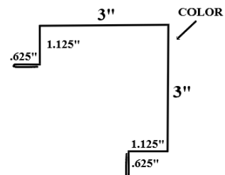
Corner Trim - Outside
