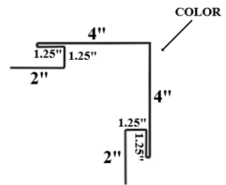
Horiz. Corner Post - Outside
