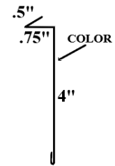
C-Flashing
