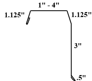
Return Eave
