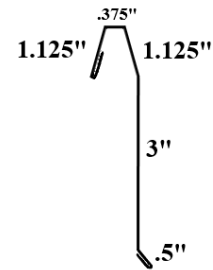
Compensating Gable
