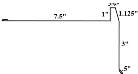
Standard Eave
