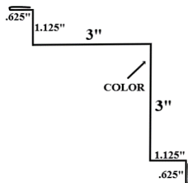
Corner Trim - Inside
